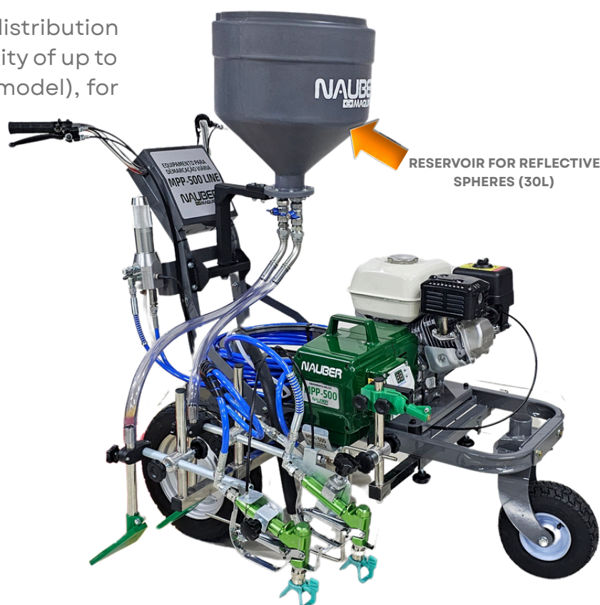
2 SPRAY GUNS FOR MARKING ON DOUBLE STRIPS
